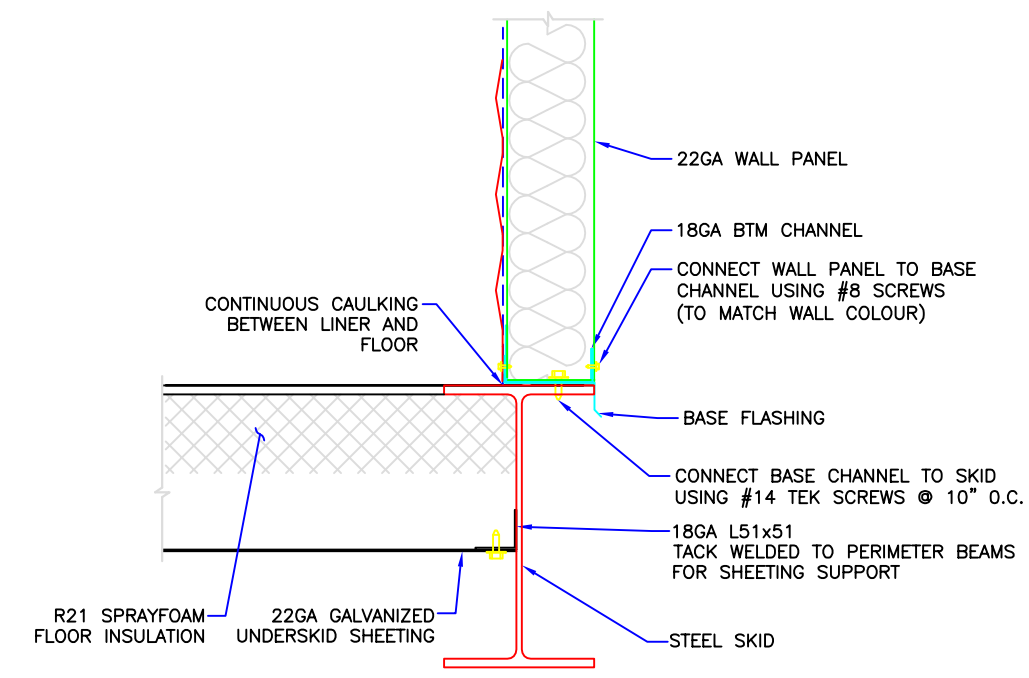
WALL TO SKID SECTION NTS
