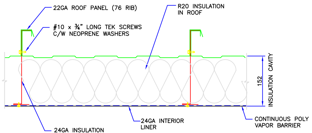
ROOF SECTION NTS
