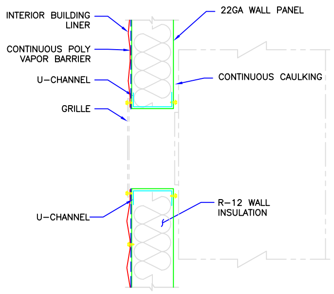
TYPICAL HVAC OPENING NTS
