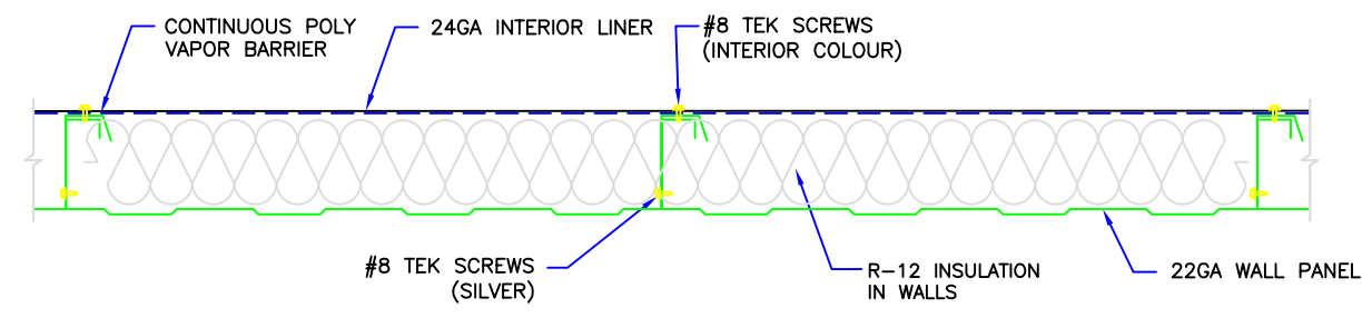
WALL SECTION NTS
