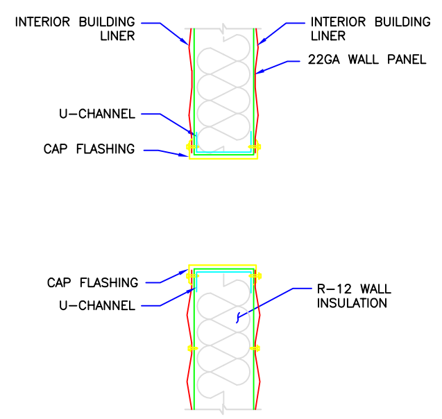
PARTITION WALL OPENING (PLAN) NTS
