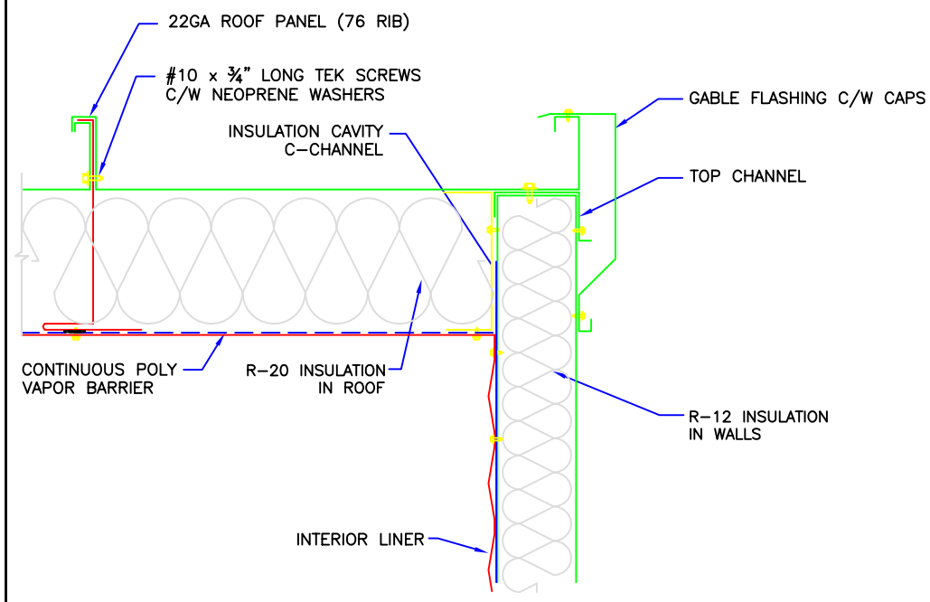
WALL ROOF CONNECTION DETAIL NTS
