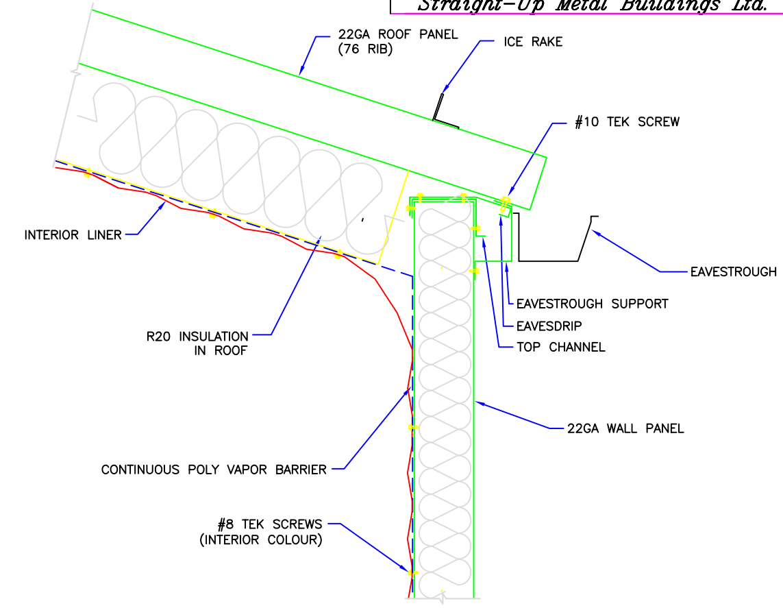
SIDE WALL SECTION NTS
